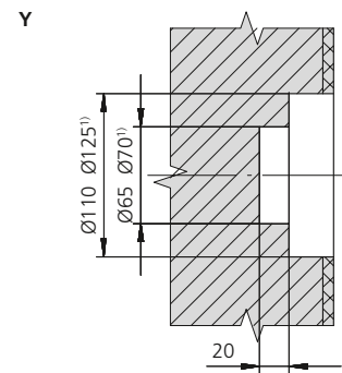
dimensions for thermoset moulds
