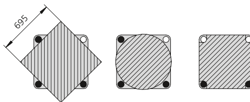
Useable mounting surface with tie bars removed
