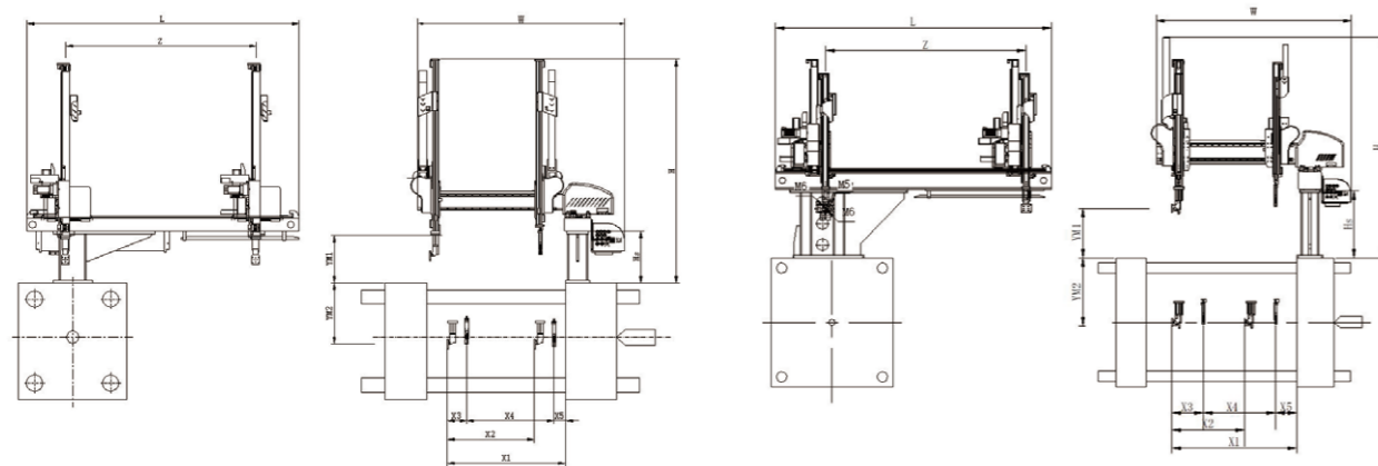
YR800S5&YR1000S5
