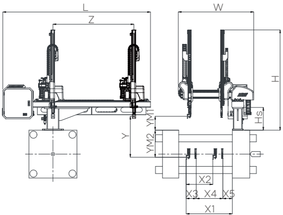
YR800S5-E & YR1000S5-E
