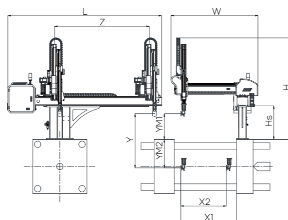
YR1000S3-DE & YR1200S3-DE
